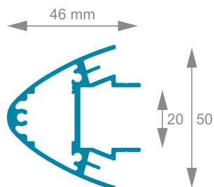
PYLON 20S
