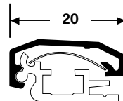
137028 (137029=VB6-A20-VOM1) C 20 mm Standaard C 20 mm Standard C 20 mm Standard
