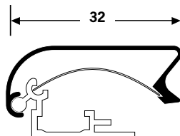
137040 (137042=VB6-A20-VOM1) 32 mm Softline 32 mm Softline 32 mm Softline
