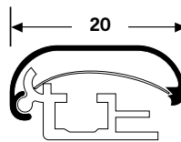
137025 (137027=VB6-A20-VOM1) 20 mm Security 20 mm Security 20 mm Security
