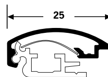
137085 (137086=VB6-A20-VOM1) C 25 mm Softline C 25 mm Softline C 25 mm Softline
