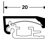
137020 (137022=VB6-A20-VOM1) 20 mm Standaard 20 mm Standard 20 mm Standard
